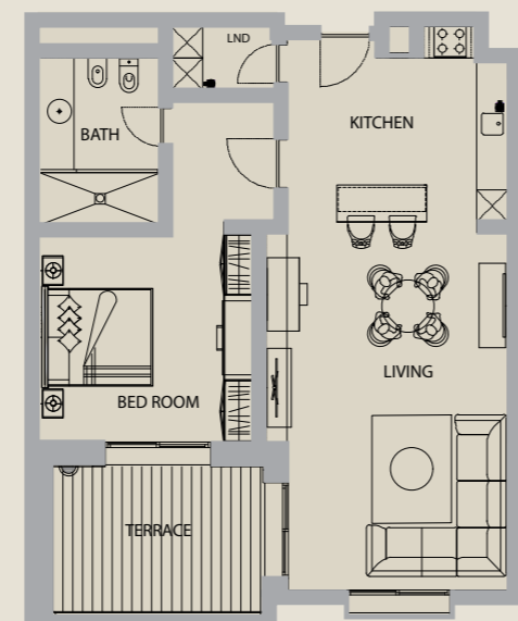
1 BED ROOM F1-08/F2-08/F3-08 LEVEL: L1/L2/L3 SELLABLE AREA 103.91 sq.m
