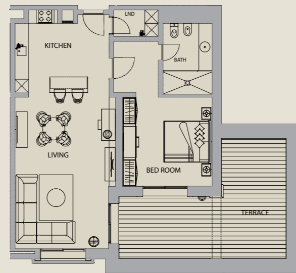
1 BED ROOM G - 05 LEVEL: GROUND
