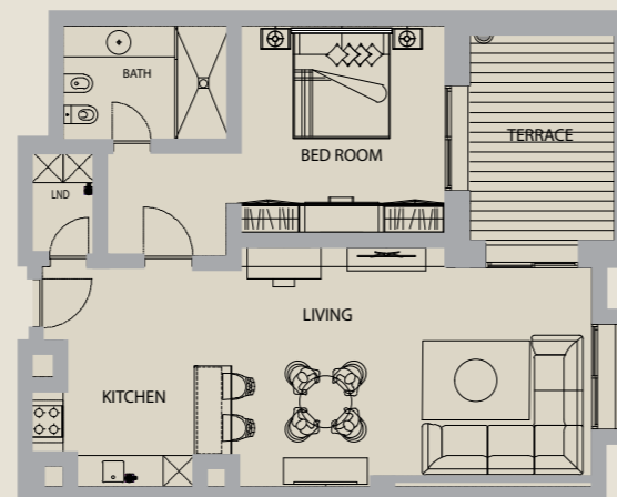
1 BED ROOM F4-14 LEVEL: L4
