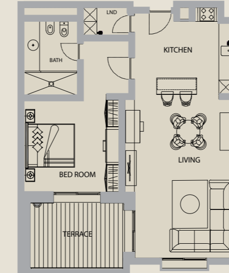
1 BED ROOM F4-06 LEVEL: L4
