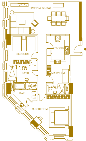
2-BDR, Unit 025, Level 2
