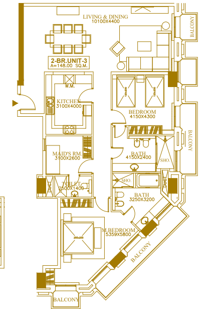
2-BDR, Unit 153, Level 15
