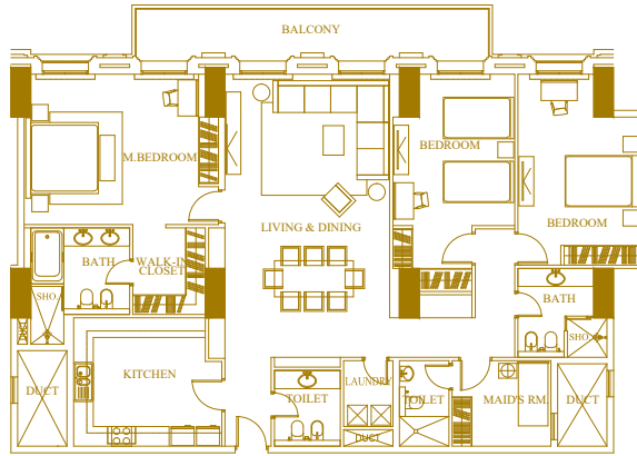
3-BDR, Unit 051, Level 5
