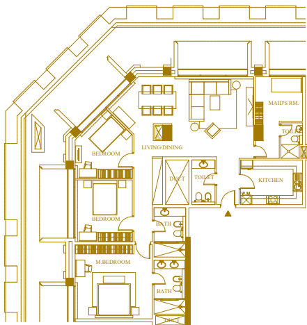
3-BDR, Unit 164, Level 16
